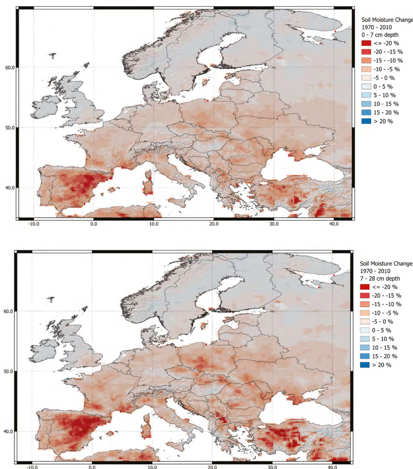
Figure 10: Change in soil moisture for 0-7cm (map above) and 7-28cm (map below) soil depths, %. 1970 vs 2010.
