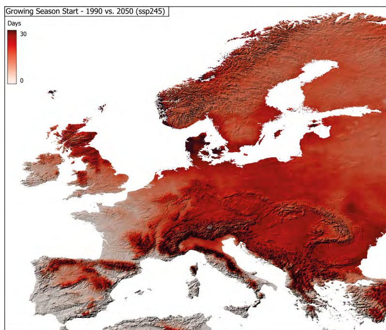
Figure 15: Growing Season Start - 1990 vs. 2050 SSP2-4.5.
