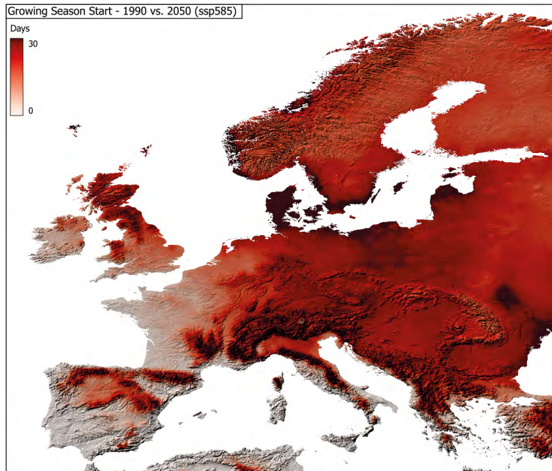
Figure 16: Growing Season Start - 1990 vs. 2050 SSP5-8.5.
