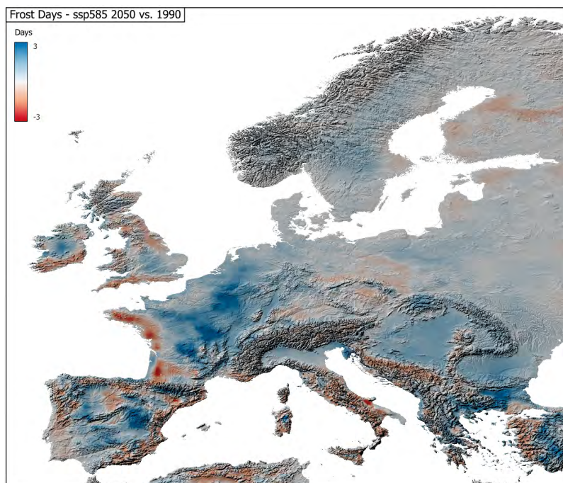
Figure 18: Change in Frost Days during growing season 1990 vs. 2050, SSP5-8.5.
